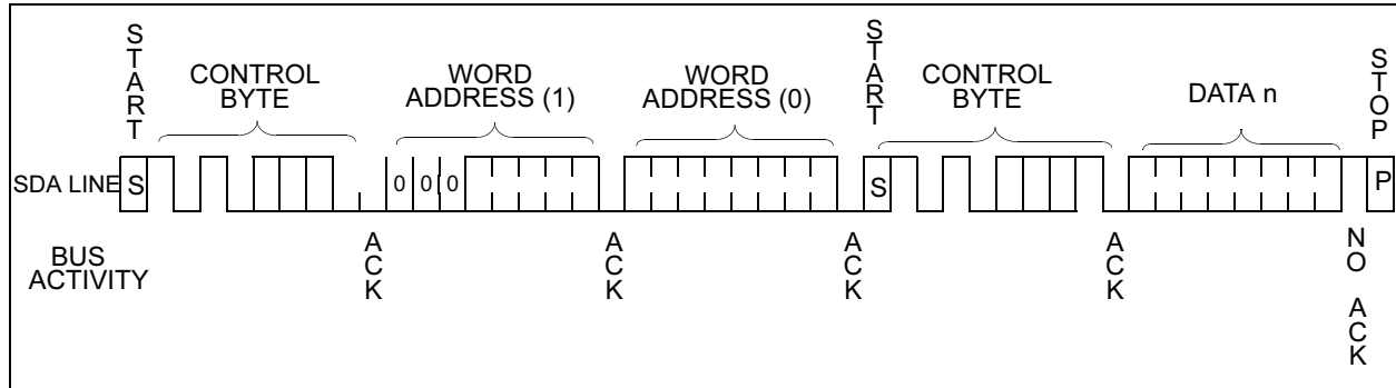
FIGURE 4-4: RANDOM READ
