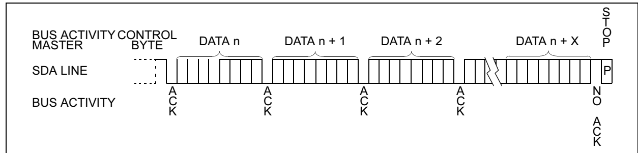
FIGURE 4-5: SEQUENTIAL READ
