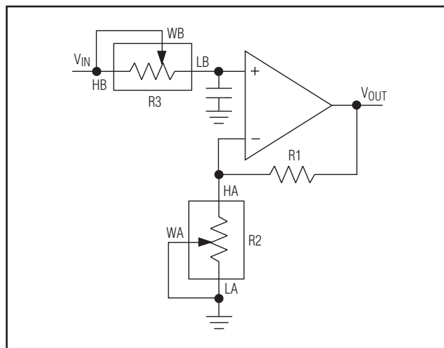
Figure 10. Programmable Filter
