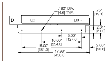
Top assembly, side view
