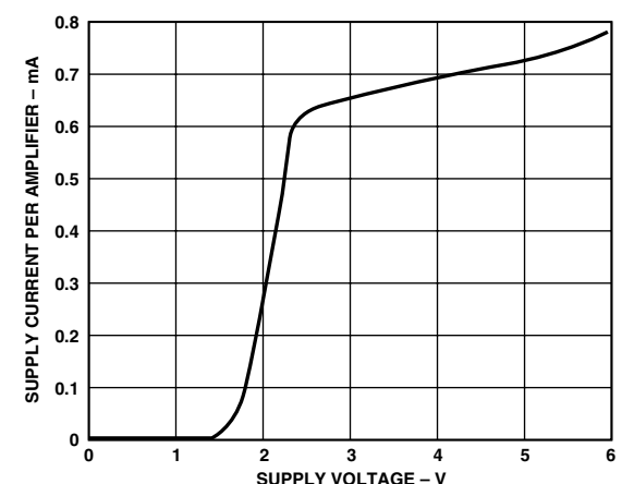
TPC 33. Supply Current per Amplifier vs. Supply Voltage
