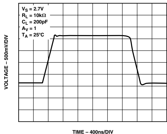
TPC 44. Large Signal Transient Response
