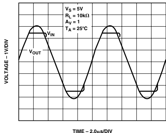
TPC 46. No Phase Reversal
