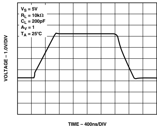
TPC 43. Large Signal Transient Response
