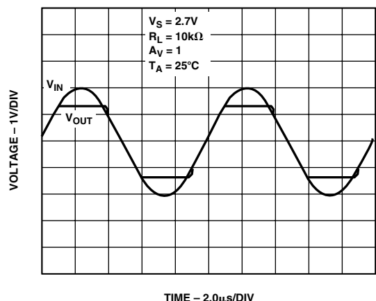
TPC 45. No Phase Reversal
