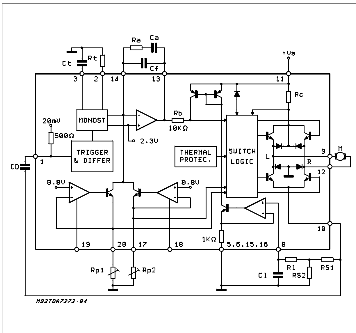
Figure 2: Application Circuit.
