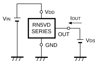
FIG. 5 Nch Driver Output Current Test Circuit
