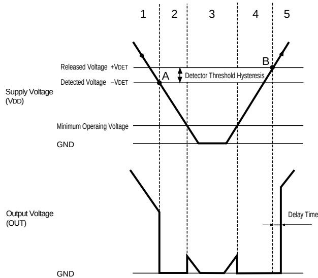
FIG. 2 Operation Diagram
