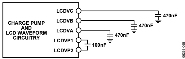
Figure 90. External Circuitry for Charge Pump Option
