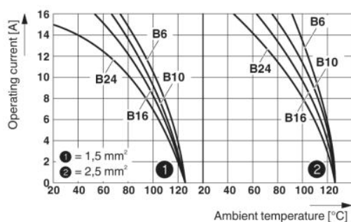
Derating diagram: Series HC-B...S / HC-B...C
