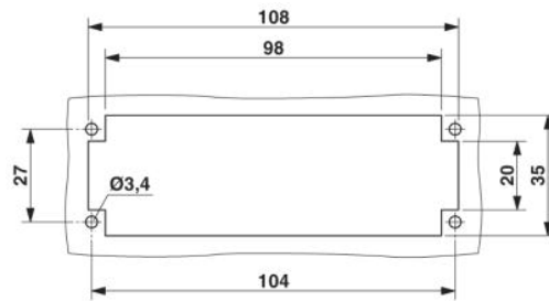
Mounting cut-out
