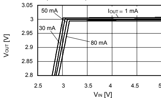
S-1111B30 ( T_a = 25^\circ\text{C} )
