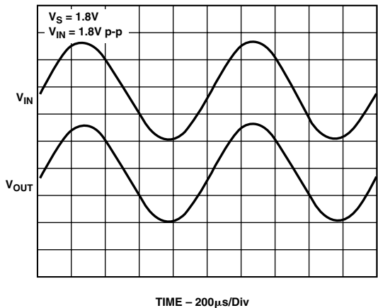
Figure 20. Rail-to-Rail Input Output
