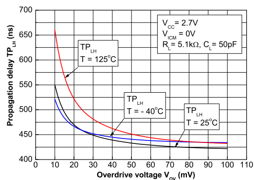
Figure 19. Propagation delay versus overdrive with positive transition, V_{CC} = 2.7V
