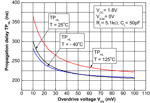
Figure 15. Propagation delay versus overdrive with negative transition, V_{CC} = 1.8V
