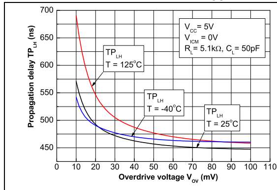
Figure 22. Propagation delay versus overdrive with positive transition, V_{CC} = 5\text{ V}
