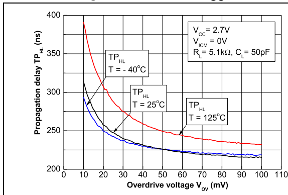
Figure 18. Propagation delay versus overdrive with negative transition, V_{CC} = 2.7V
