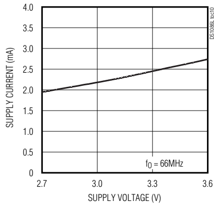
SUPPLY CURRENT WITH OUTPUT DISABLED vs. SUPPLY VOLTAGE
