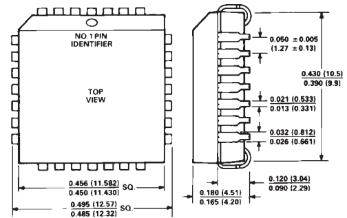
28-Pin PLC (P-28A)
