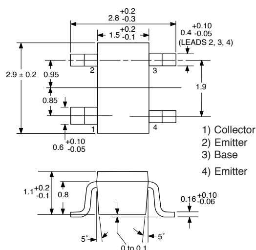
PACKAGE OUTLINE 39
