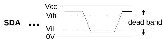
Figure 10. SDA/SCL Levels
