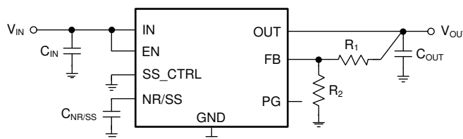
Figure 38. Adjustable Operation
