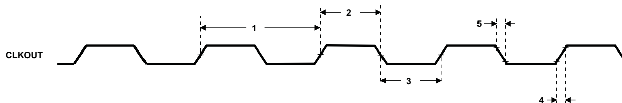
Figure 6-10. CLKOUT Timing
