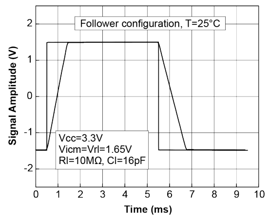
Figure 17. Desaturation time
