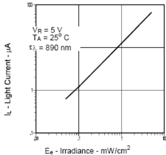
Light Current vs. Irradiance
