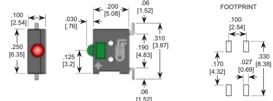
Figure 3. Vertical Indicator
