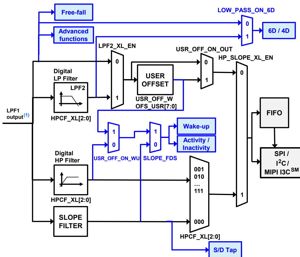
Figure 27. Accelerometer block diagram
