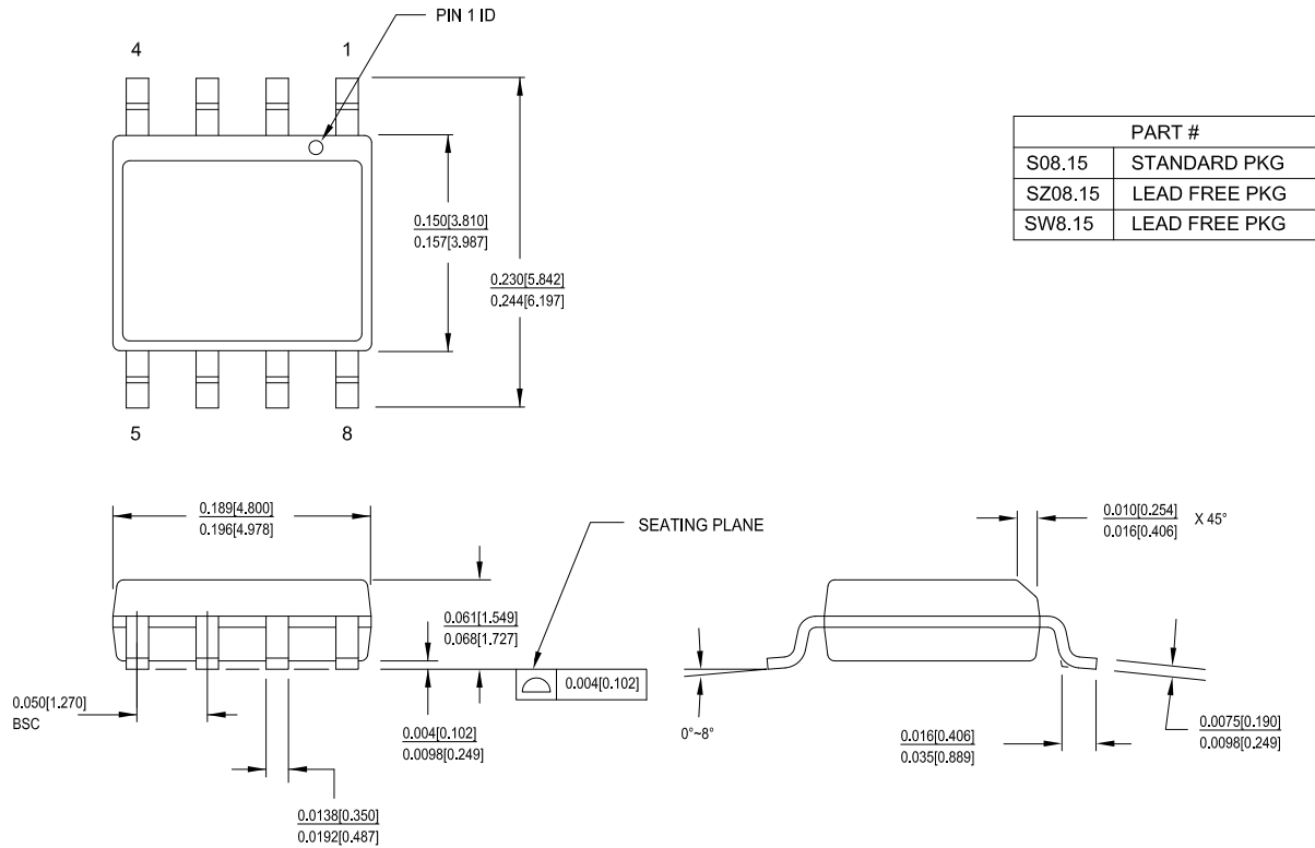
Figure 36. 8-pin SOIC (150 Mils) S0815/SZ815/SW815 Package Outline, 51-85066
