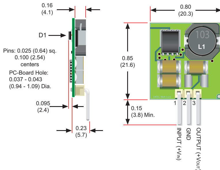
Horizontal Package (H Pin Option)
