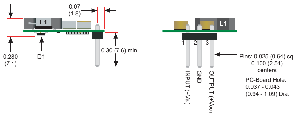
Horizontal Package (H Pin Option)
