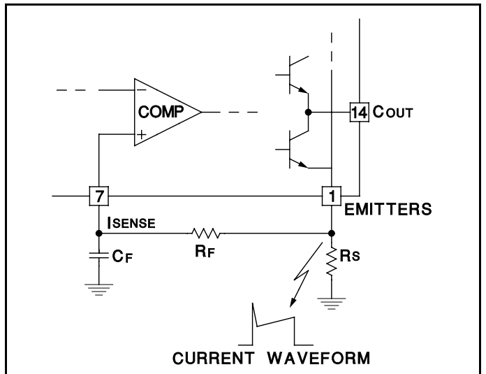
Figure 1. Current Sense Filter
