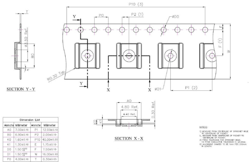
Figure 17. Carrier Tape for HTSSOP20 20L
