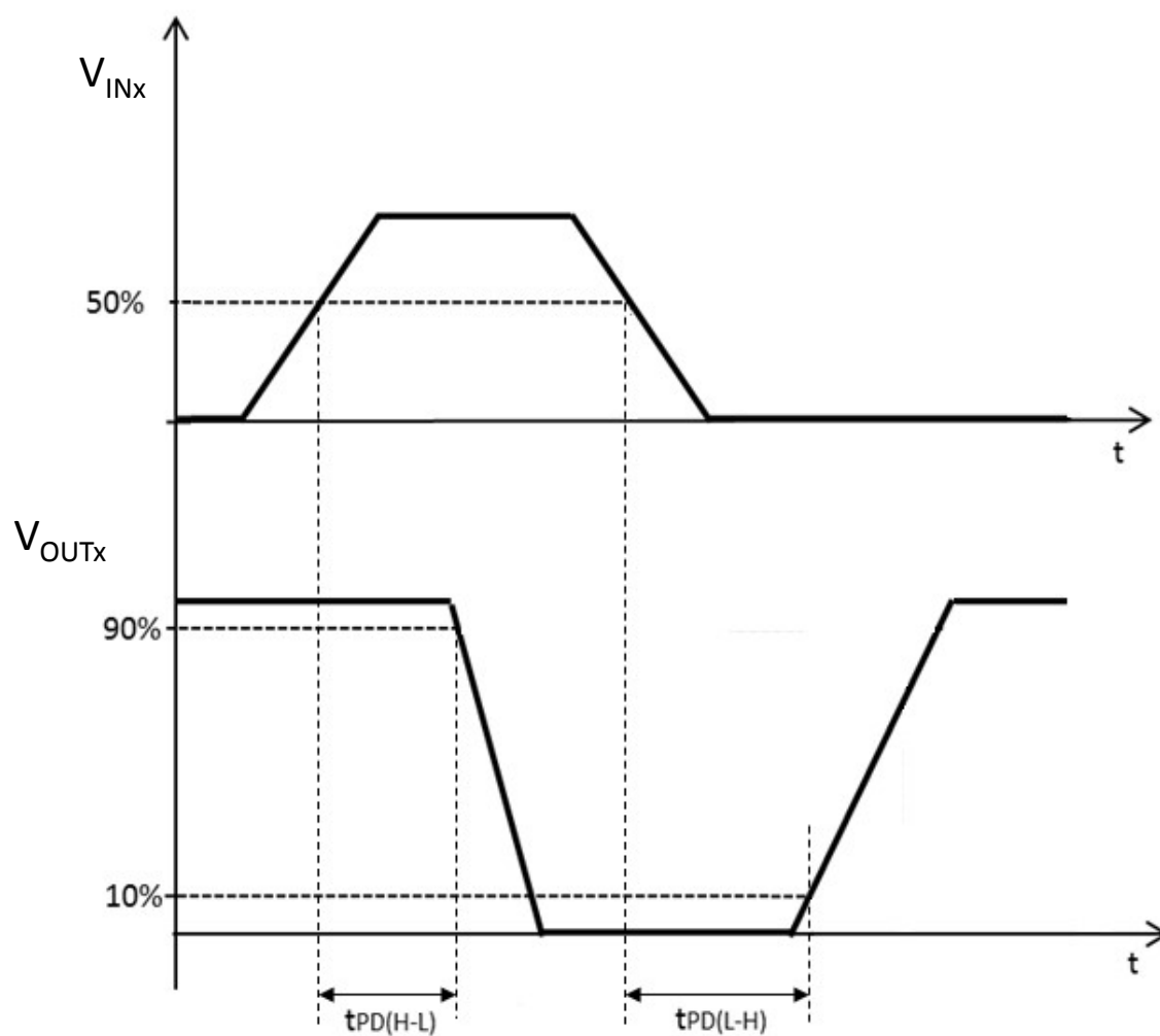
Figure 4. t_{PD(L-H)} and t_{PD(H-L)}
