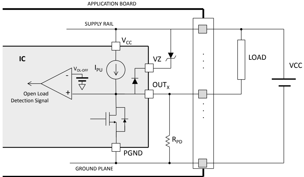
Figure 10. Open load off-state
