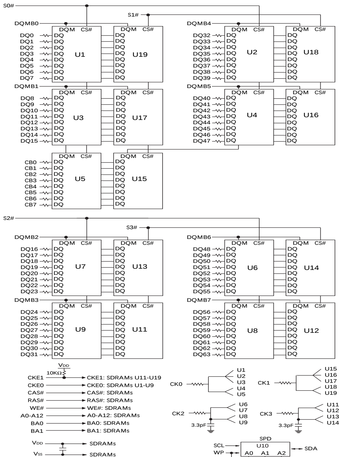
Figure 4: Functional Block Diagram – Dual Rank
