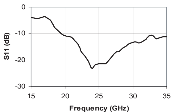
Figure 3. Input Return Loss
