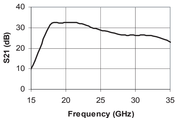
Figure 1. Small-signal Gain
