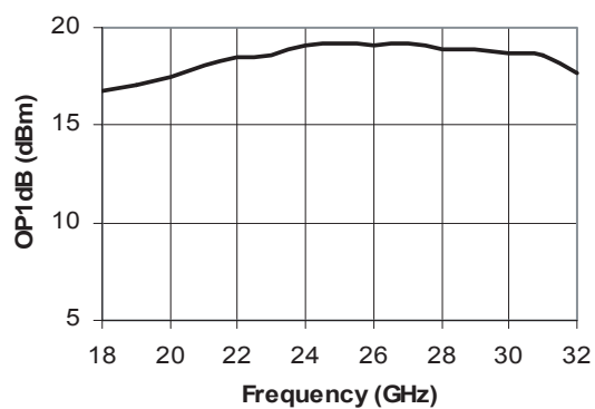
Figure 4. Output P-1dB
