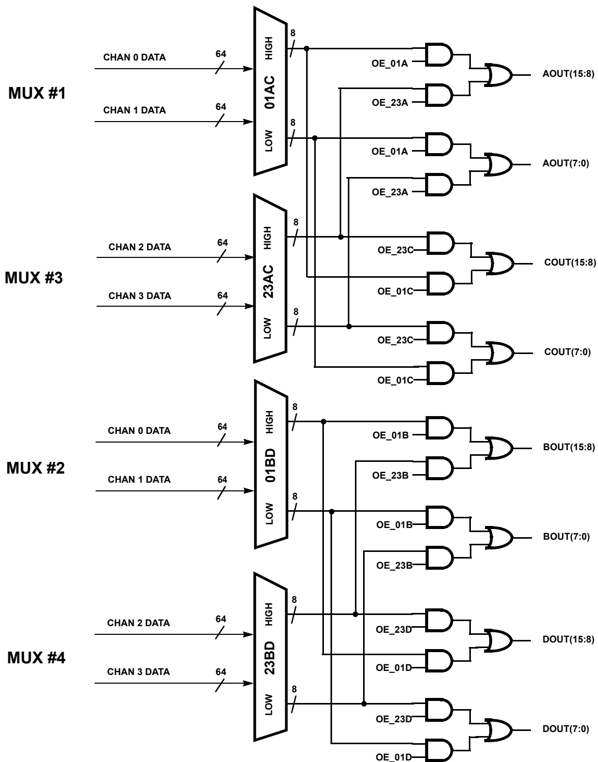
FIGURE 10. OUTPUT ROUTING
