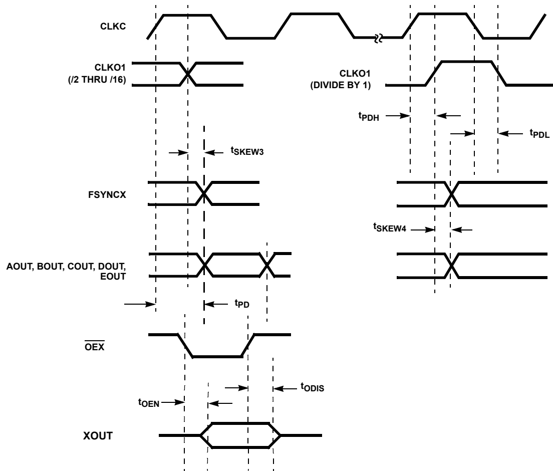
FIGURE 18. OUTPUT TIMING
