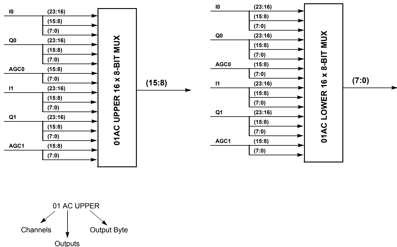
FIGURE 9. MULTIPLEXING CHANNELS
