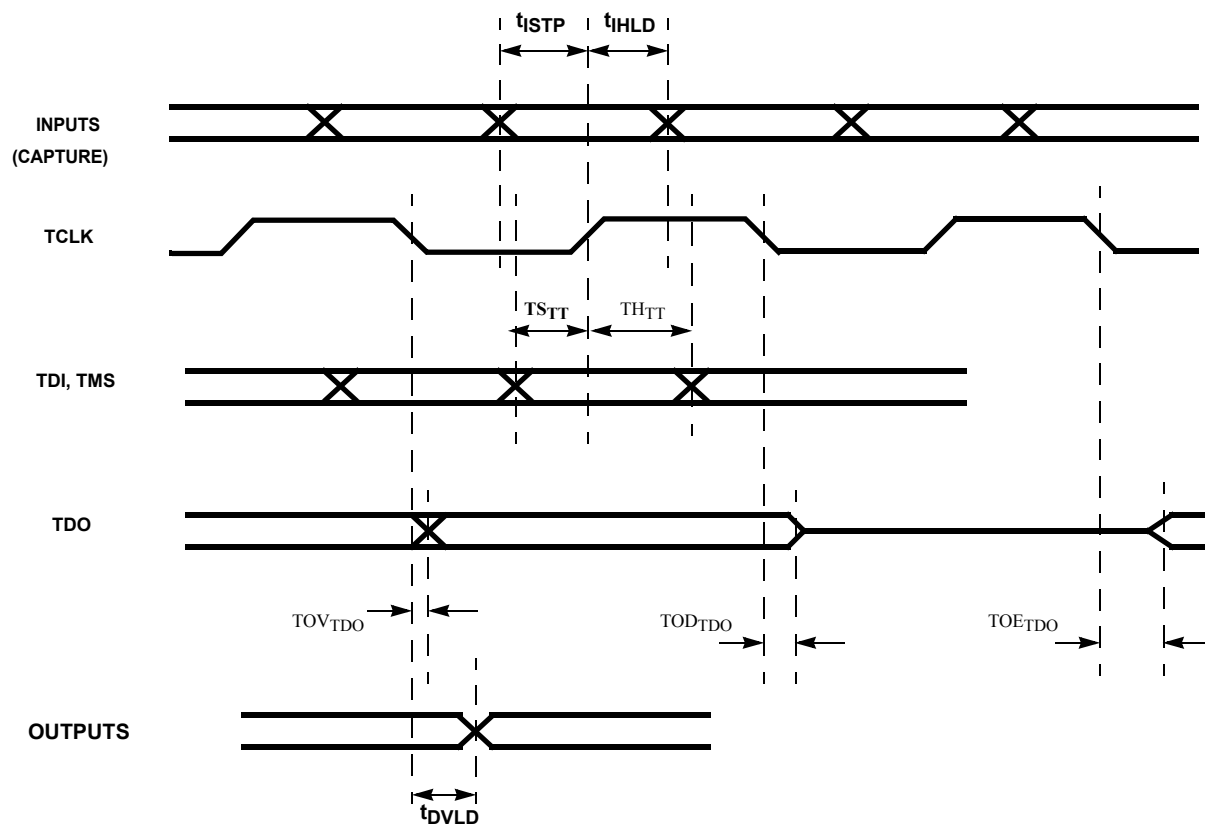
FIGURE 17. JTAG TIMING
