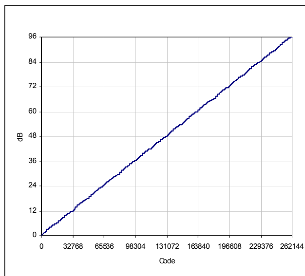
FIGURE 5A. ISL5416 AGC FORWARD GAIN RESPONSE
