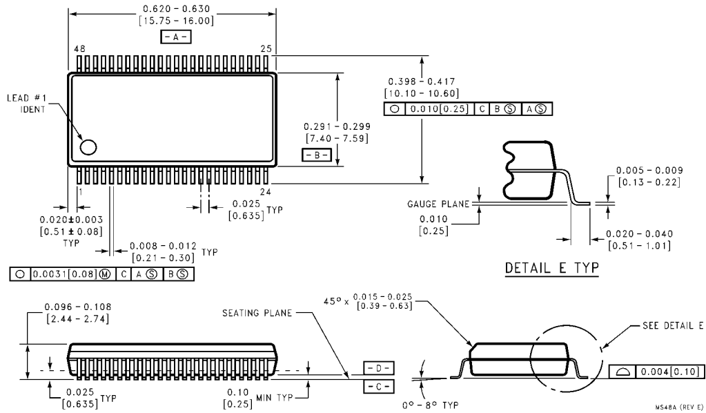
48-Lead Small Shrink Outline Package (SSOP), JEDEC MO-118, 0.300" Wide Package Number MS48A
