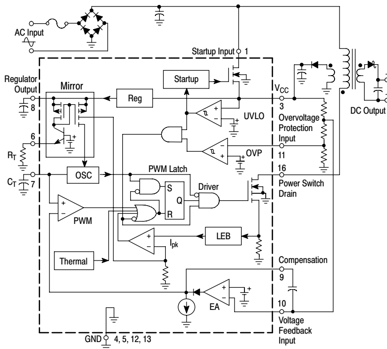
Figure 1. Simplified Application
