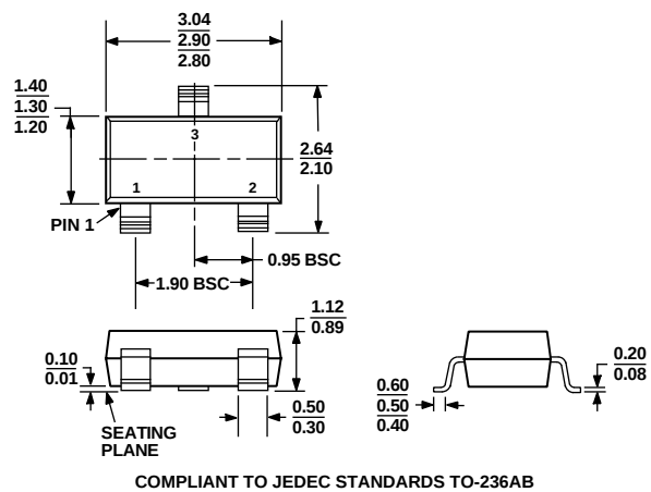
Figure 25. Surface-Mount Package[SOT-23]
