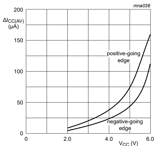
Fig. 11. \Delta I_{\text{CC(AV)}} as a function of V_{\text{CC}} for 74HC2G17-Q100
