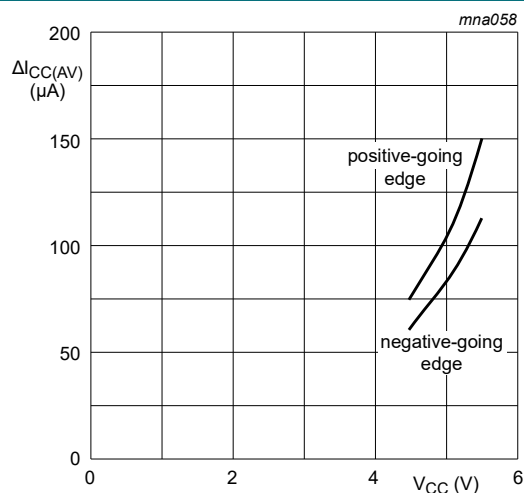
Fig. 12. \Delta I_{\text{CC(AV)}} as a function of V_{\text{CC}} for 74HCT2G17-Q100
