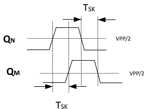
Output-Output Skew
