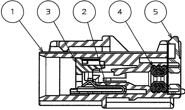
SECT. A-A
