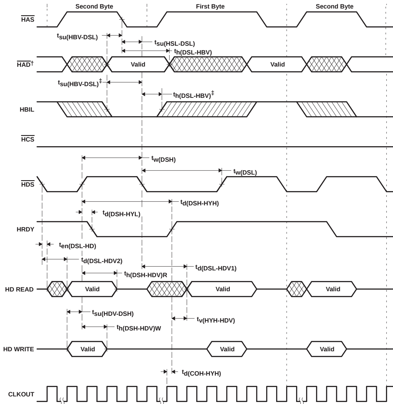
Figure 5-27. Using \overline{\text{HDS}} to Control Accesses ( \overline{\text{HCS}} Always Low)
