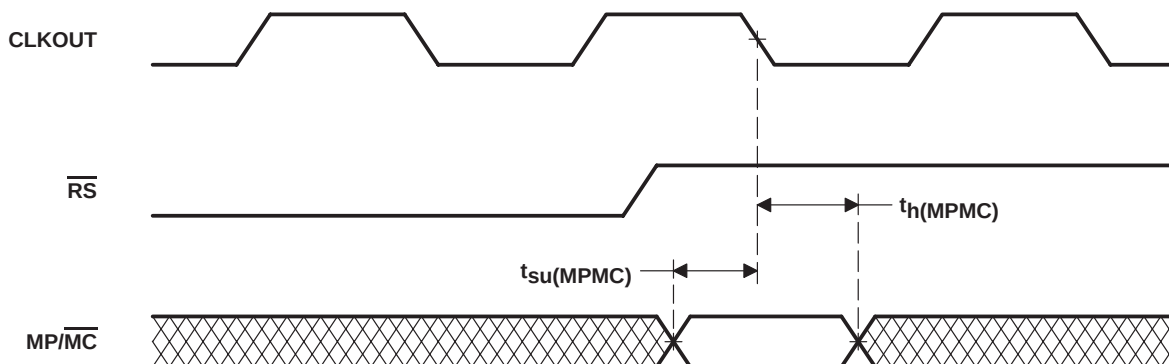
Figure 5-16. \overline{MP/MC} Timing
