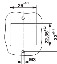
Panel cutout
