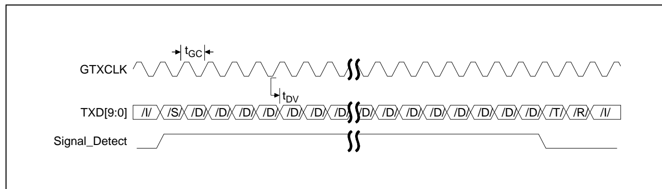
Note1: These measurements were obtained through simulation and lab measurement using a 10pF load. See ZL5011x Design Manual section “7.1.3.1 TBI Interface Timing” for proper operation when using the TBI interface.
