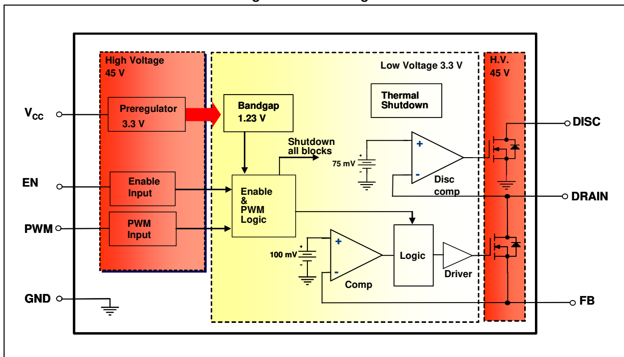
Figure 4. Block diagram
