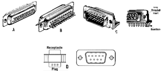
.318 (Footprint) Right Angle PCB with 4-40 Thread (Plug) — Fig. C
