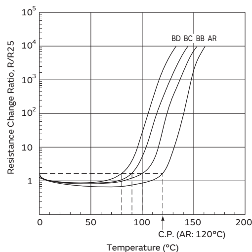
Resistance-Temperature Characteristic
