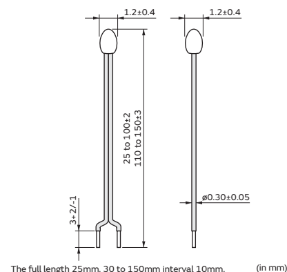
NXFS15_2B Type (without twist)
