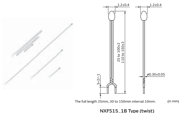
NXFS15_1B Type (twist)
