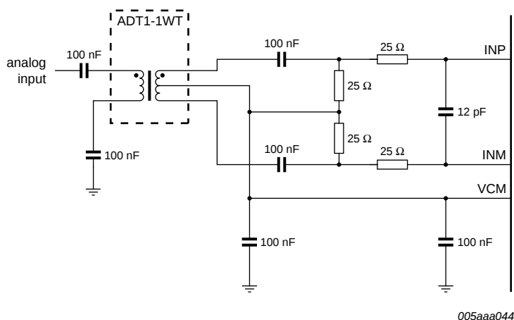
Fig 8. Single transformer configuration
