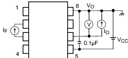
Fig. 12.1.1 I_{OPH} Test Circuit
