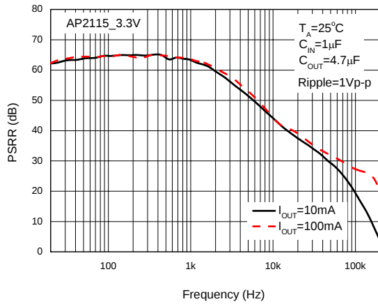
Figure 24. PSRR vs. Frequency
