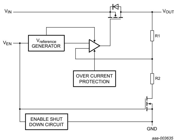
Fig 3. Block diagram of LD6815TD/xxH
