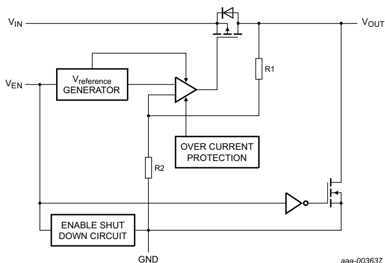
Fig 2. Block diagram of LD6815TD/xxP (auto discharge function)
