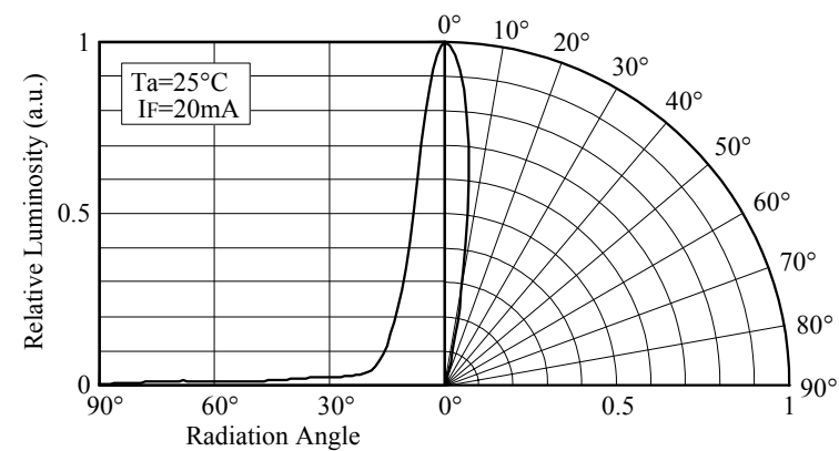
■ Directivity (NSPG500(S))
