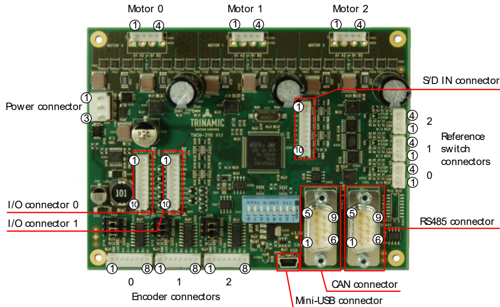
Figure 3.2 TMCM-3110 connectors
