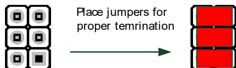
Figure 3.4 Encoder input termination
