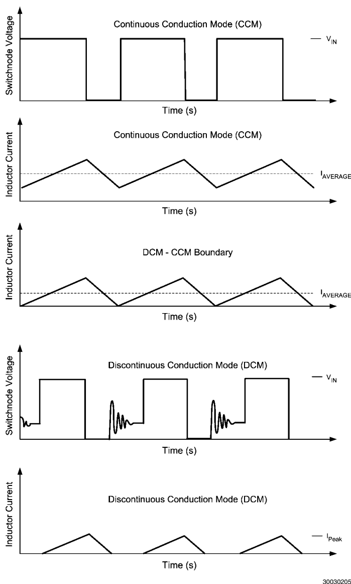
FIGURE 1. Modes of Operation for LM20125
