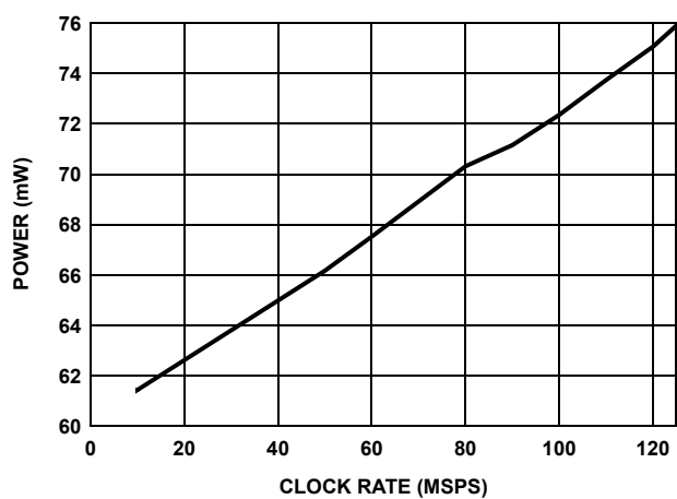
FIGURE 38. POWER vs CLOCK RATE, f_{CLK}/f_{OUT} = 10 , I_{OUT} = 20\text{mA}
