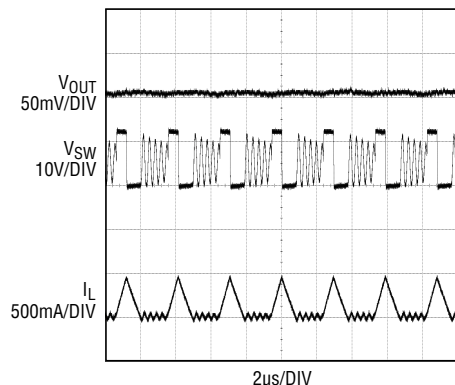
Pulse-Skipping Mode Operation Waveforms
