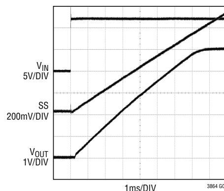
Normal Soft Start-Up
