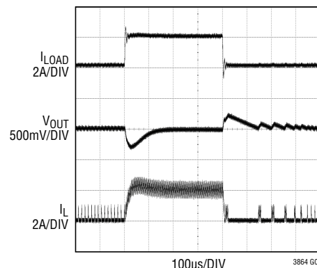
Transient Response: Burst Mode Operation
