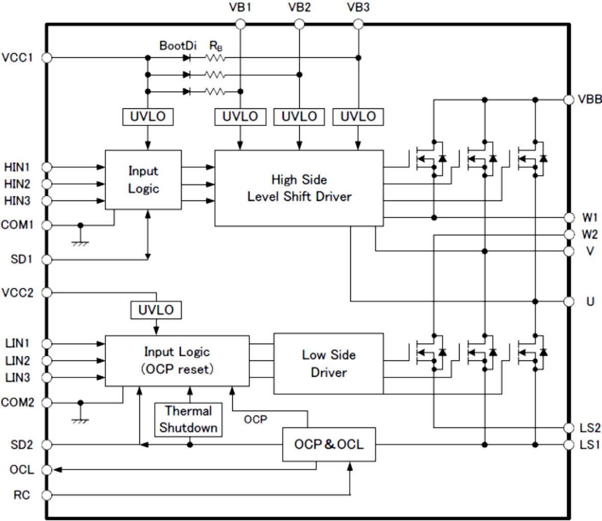
Pin-out Diagrams
